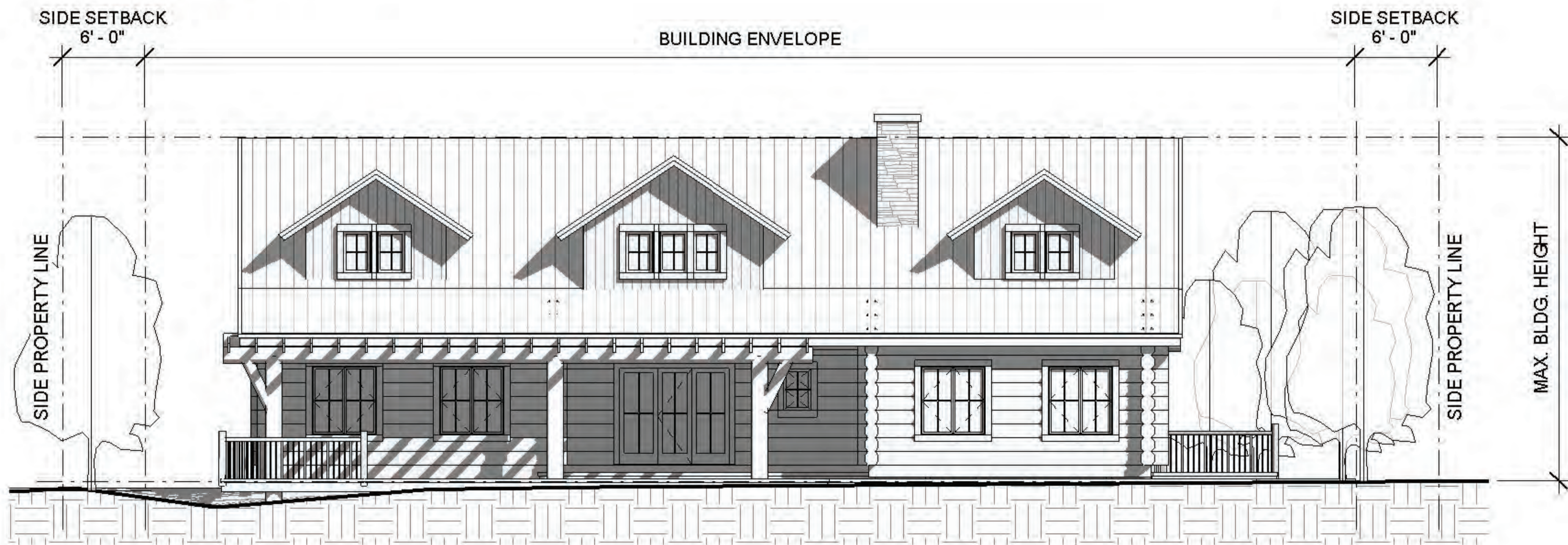
3 REAR ELEVATION 1" = 10'-0"
